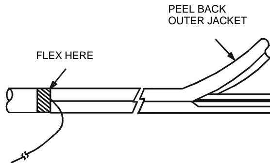
Figure 5 - Remove the outer cable jacket to expose core tube
